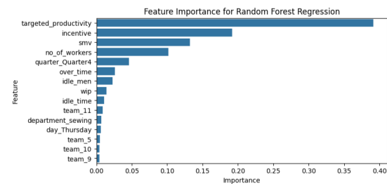
Fig. 9. Random forest feature importance.
